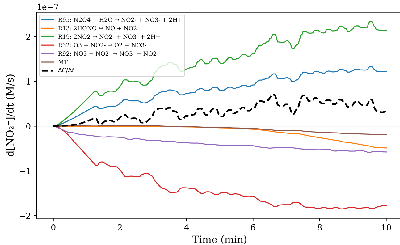
(c) \text{NO}_2^-
